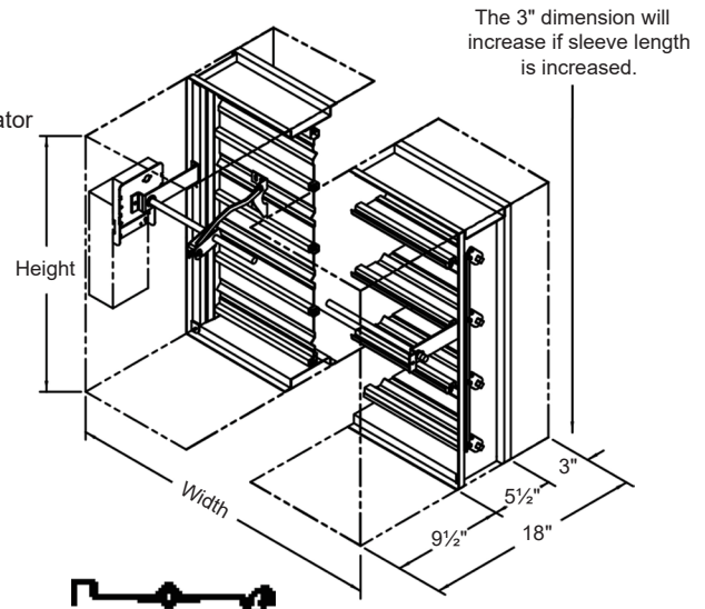
Blade Profile
